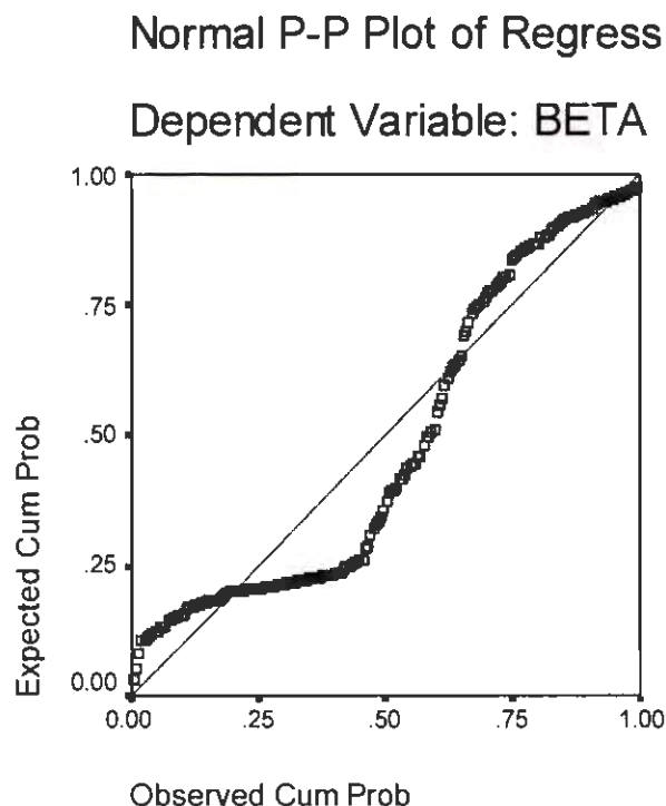
Gambar 4.1. Normal P-P Plot of Regression Standard
